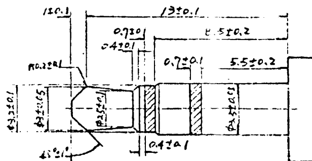
3.5 MATE PLUG
